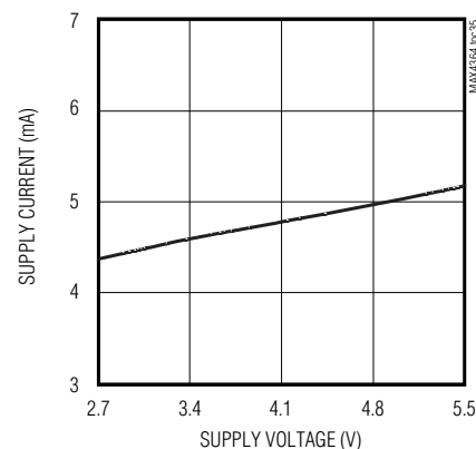
MAX4365 SUPPLY CURRENT vs. SUPPLY VOLTAGE
