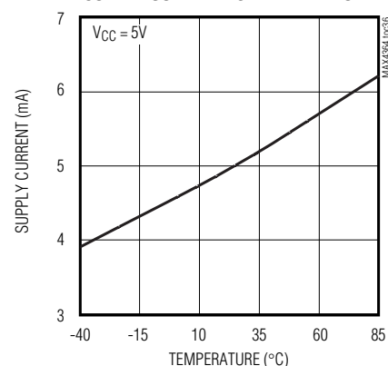
MAX4365 SUPPLY CURRENT vs. TEMPERATURE
