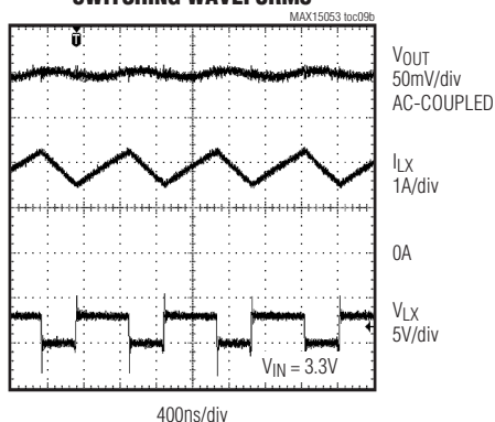
SWITCHING WAVEFORMS
