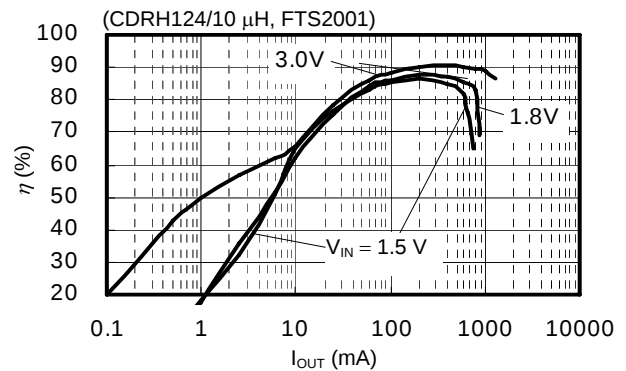
(20) S-8341C33AFT
