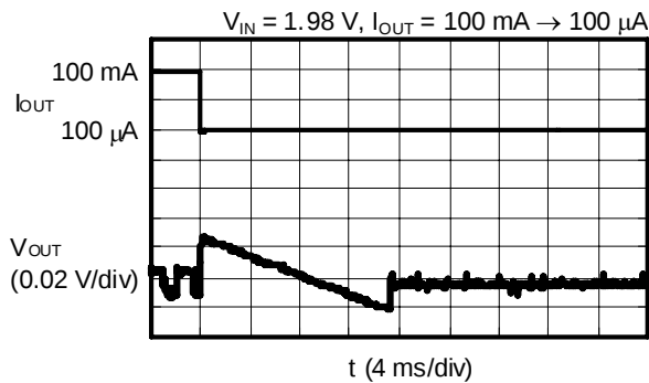
S-8340A33AFT, f_{OSC} = 600 \text{ kHz}
