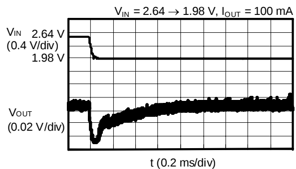
S-8340C33AFT, f_{OSC} = 300 \text{ kHz}
