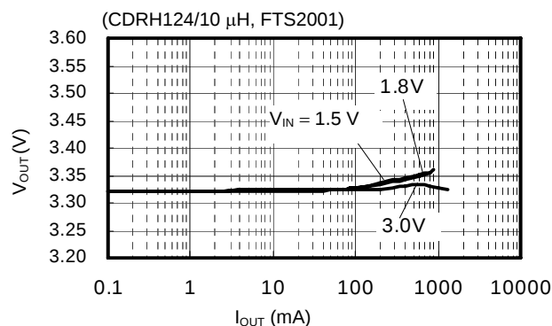
(20) S-8341C33AFT
