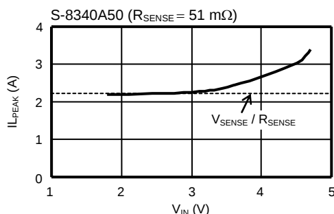
Figure 12 I_{\text{LPEAK}} Measured at Activation of Current Limit ( V_{\text{OUT}} Starts to Fall)
