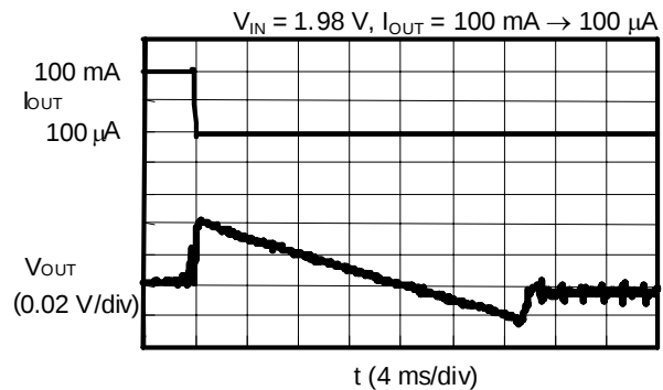
S-8340C33AFT, f_{OSC} = 300 \text{ kHz}
