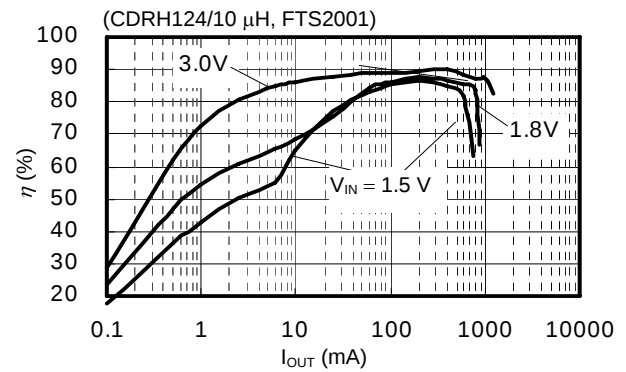
(22) S-8340C50AFT
