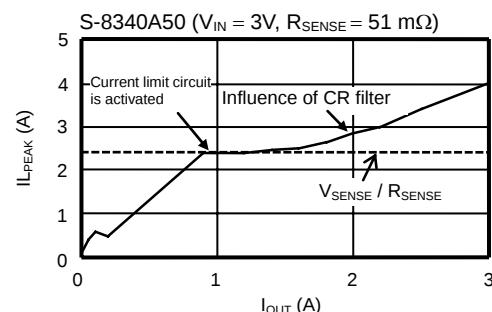
Figure 13 Measuring Coil Peak Current ( I_{\text{LPEAK}} )
