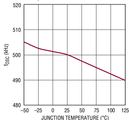
Oscillator Frequency f_{OSC} vs Temperature
