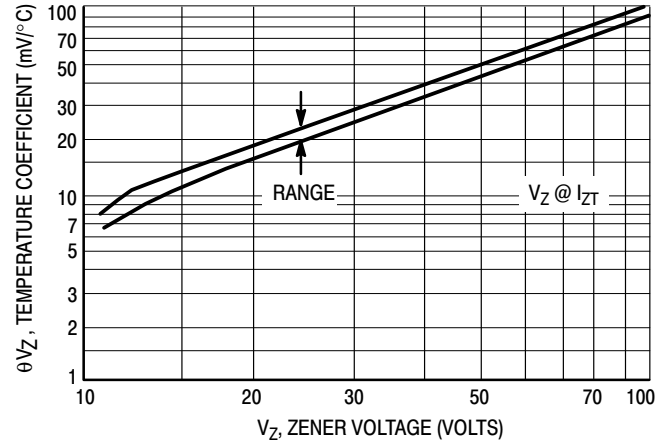
Figure 2. Temperature Coefficients
