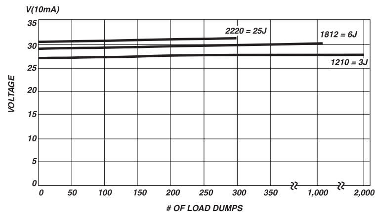
FIGURE 6. REPETITIVE LOAD DUMP PULSING AT RATED ENERGY
