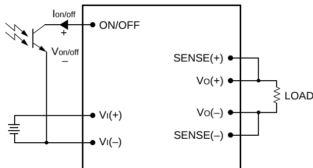
Figure 10. Remote On/Off Implementation
