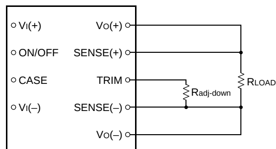
Figure 12. Circuit Configuration to Decrease Output Voltage
