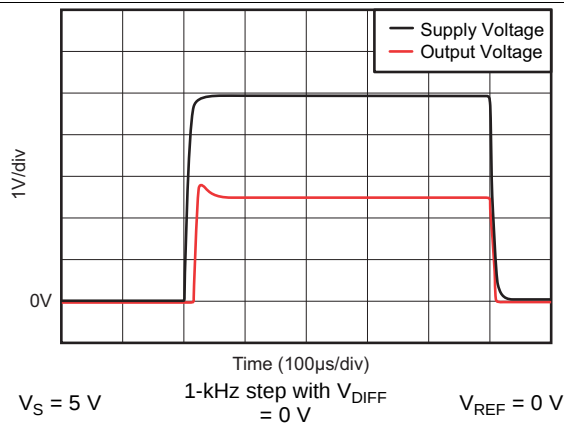
Figure 21. Start-Up Response
