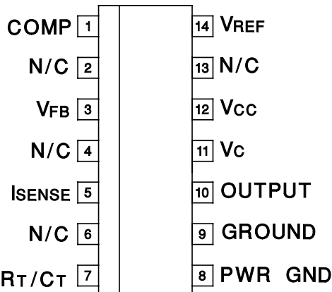
SOIC-14 (TOP VIEW) D Package
