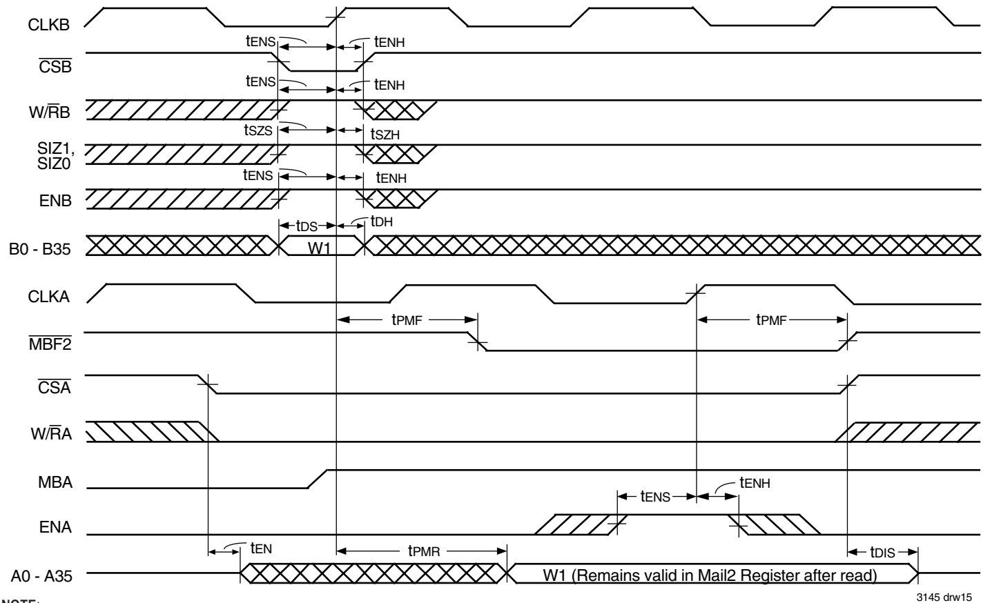
Figure 15. Timing for Mail2 Register and \overline{MBF2} Flag
