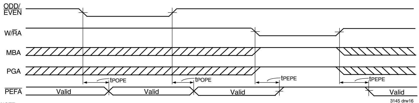
Figure 16. ODD/ \overline{EVEN} , \overline{W/RA} , MBA, and PGA to \overline{PEFA} Timing
