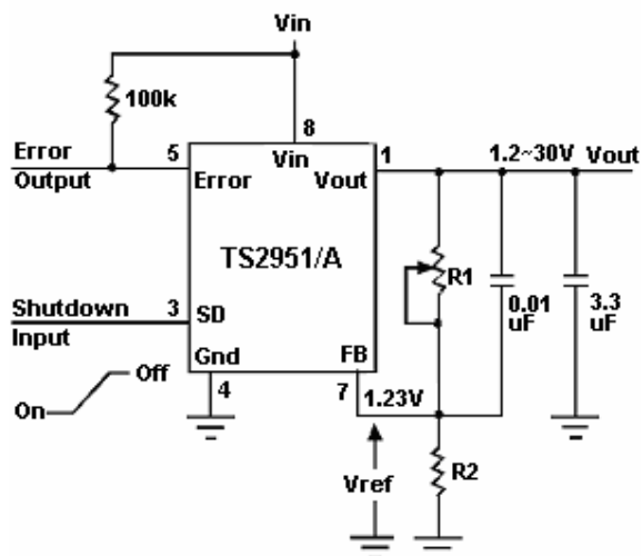
Figure 2. Adjust Voltage
