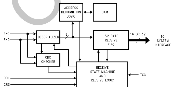
FIGURE 3-6. MAC Receiver
