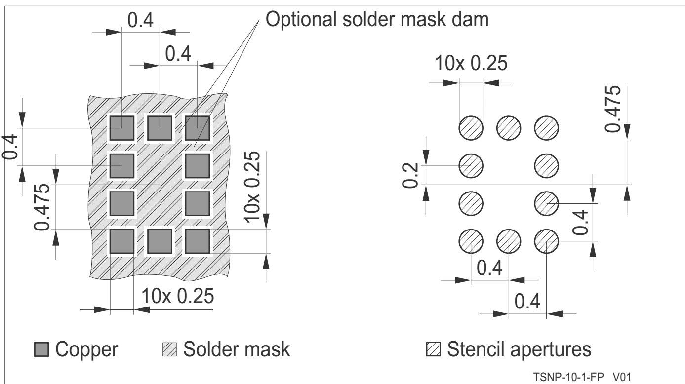
Figure 4: Land pattern and stencil mask
