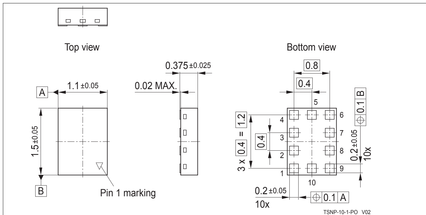
Figure 3: Package Dimensions Drawing
