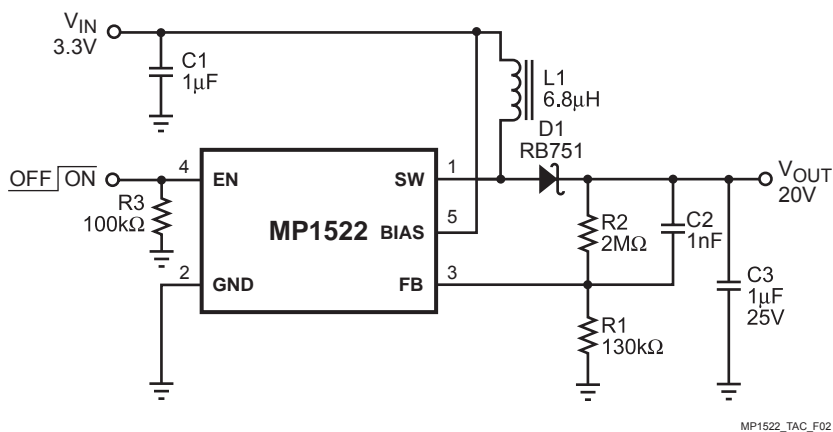
Figure 2—Typical Boost Application
