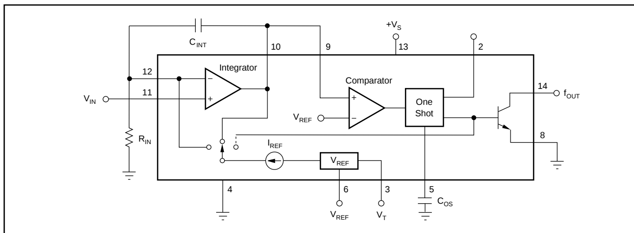
FIGURE 1. VFC121 Architecture.
