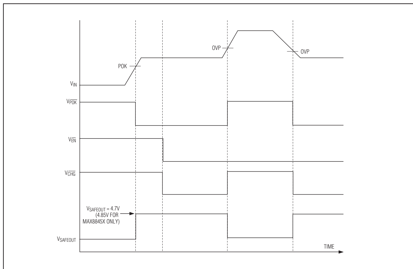
Figure 6. Timing Diagram
