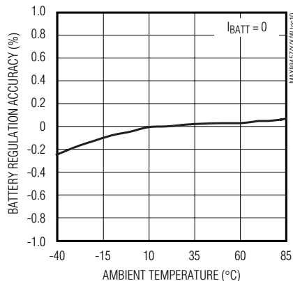
BATTERY REGULATION ACCURACY vs. AMBIENT TEMPERATURE
