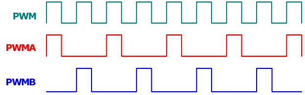
FIGURE 4. INTERLEAVING MODE'S OPERATIONAL WAVEFORMS ( EN_x = V_{CC} , OR 81\% \cdot V_{CC} )
