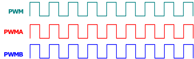
FIGURE 5. SYNCHRONOUS MODE'S OPERATIONAL WAVEFORMS ( EN\_PH\_SYNC = 60\% \cdot V_{CC} )
