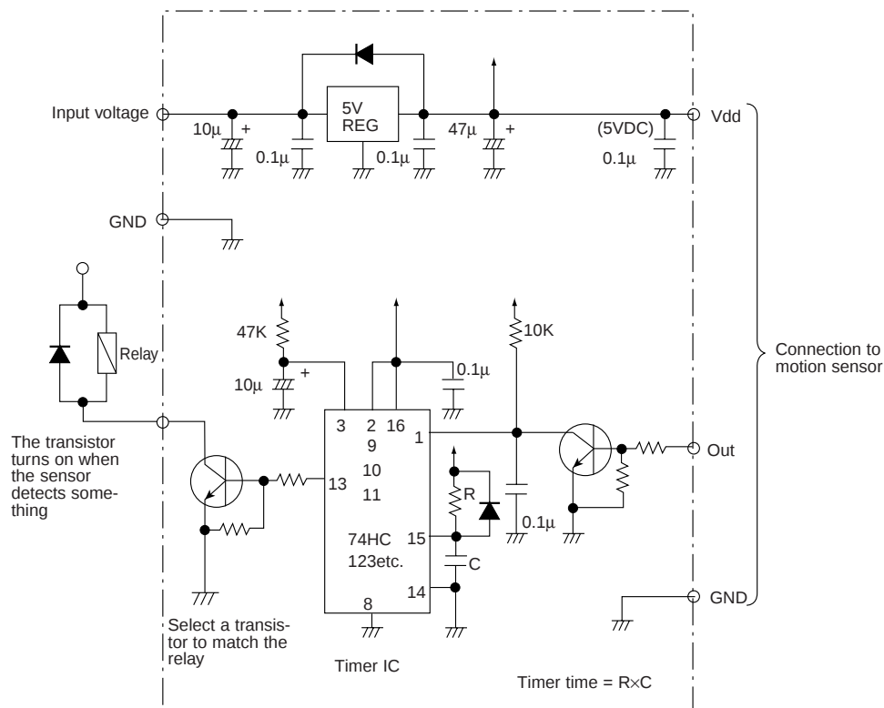
Example of a relay drive circuit using a timer circuit
