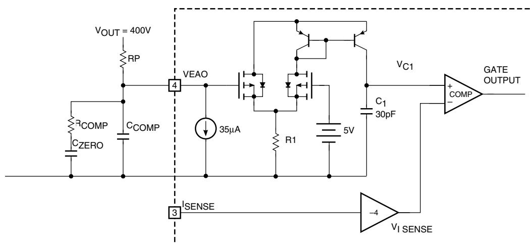
Figure 11. ML4803 PFC Control
