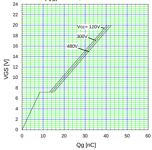
Typical Gate Charge Characteristics V GS =f(Q g ):I D =3A, T ch =25°C
