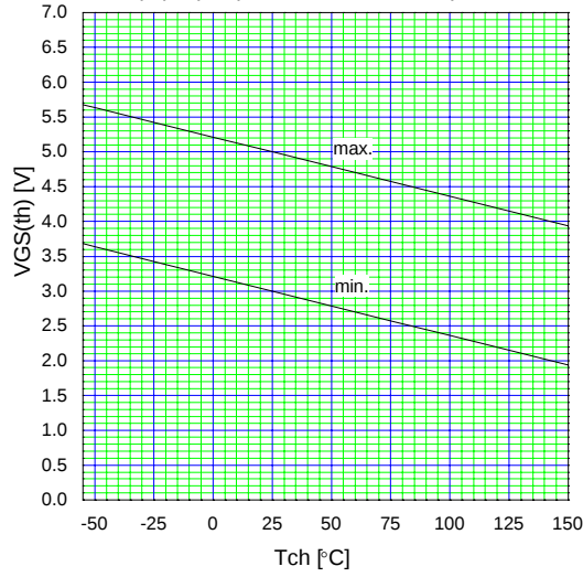
Gate Threshold Voltage vs. T ch V GS(th) =f(T ch ):V DS =V GS ,I D =250μA
