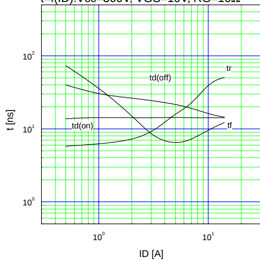
Typical Switching Characteristics vs. I D t=f(I D ):V CC =300V, V GS =10V, R G =10Ω
