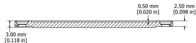
SECTION C-C
