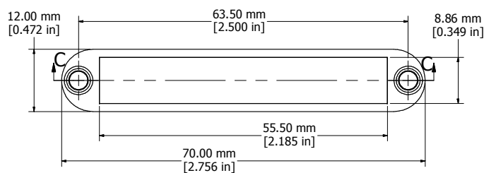
CLOSED BEZEL
