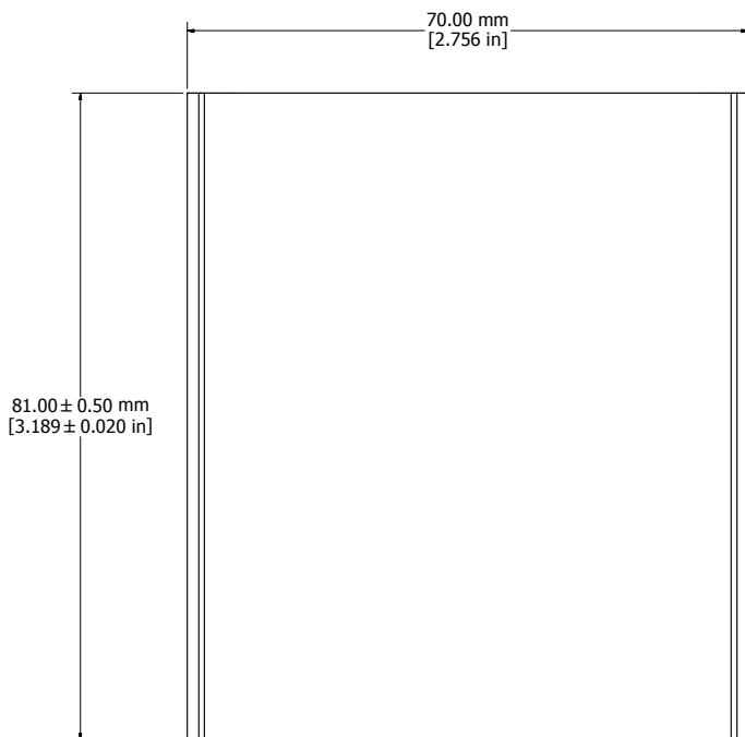
EXTRUSION
