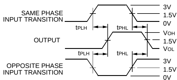
Propagation Delay
