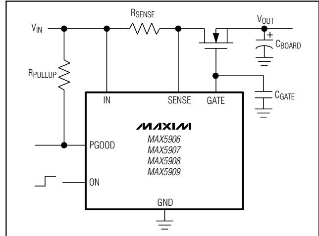
Figure 4. Operating with an External Gate Capacitor
