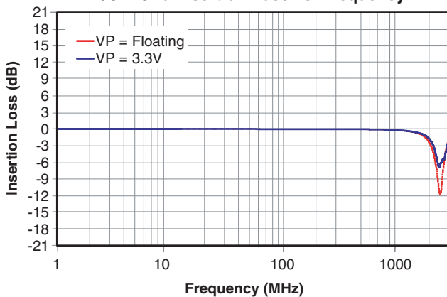
I/O – Gnd Insertion Loss vs. Frequency
