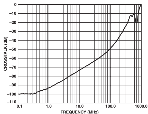
TPC 10. AD8187 All Hostile Crosstalk* vs. Frequency
