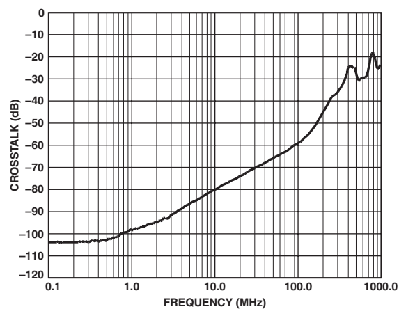
TPC 11. AD8187 Adjacent Channel Crosstalk* vs. Frequency
