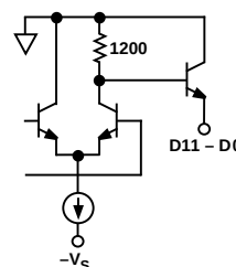
AD9027 Output Stage
