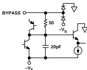
Bypass
