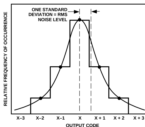
Figure 22. ADC Equivalent Input Noise
