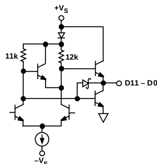
AD9026 Output Stage
