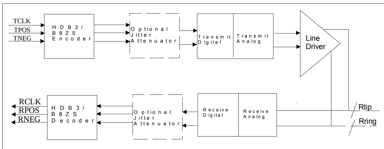
Figure 6-8. Analog Loopback
