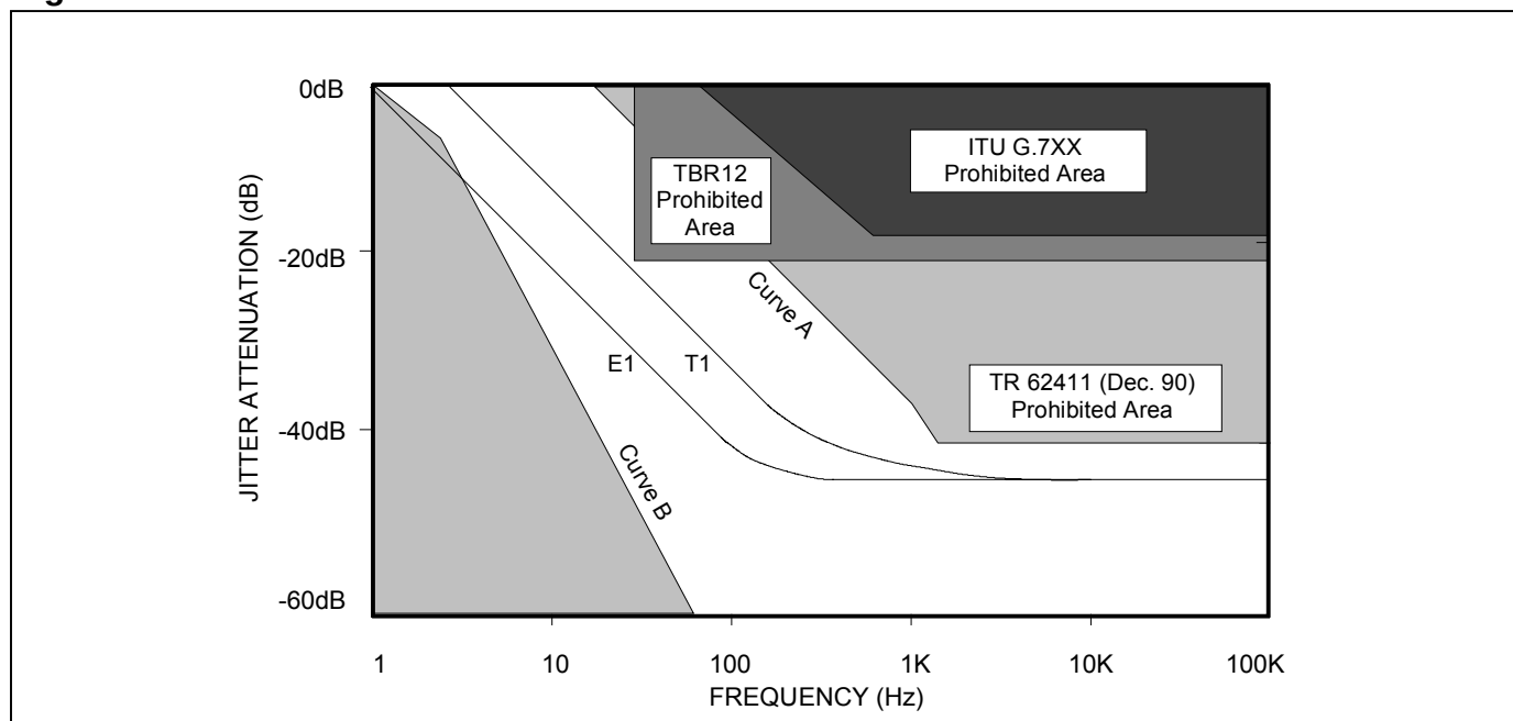
Figure 6-7. Jitter Attenuation
