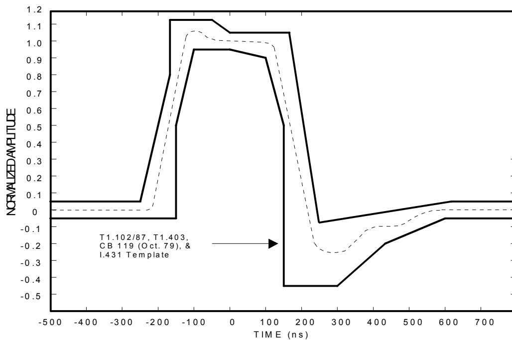
Figure 6-2. T1 Transmit Pulse Templates
