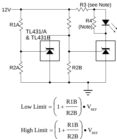
Figure 20 – Voltage Monitor
