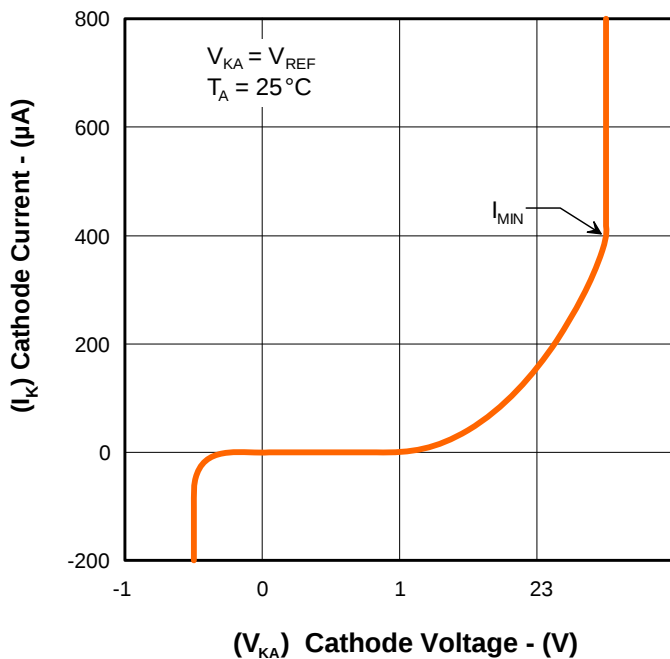
Figure 4 – Cathode Current vs. Cathode Voltage
