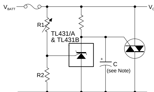
Figure 19 – Crowbar Circuit
