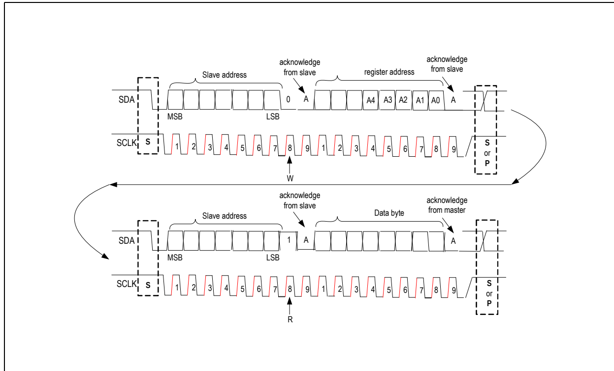
Figure 25. I 2 C Read Operation
