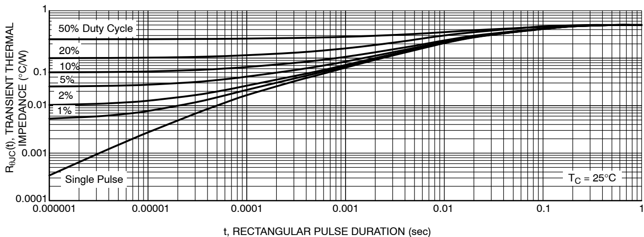
Figure 13. Thermal Response
