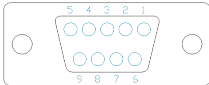
Figure 10: Serial DB9 Connector
