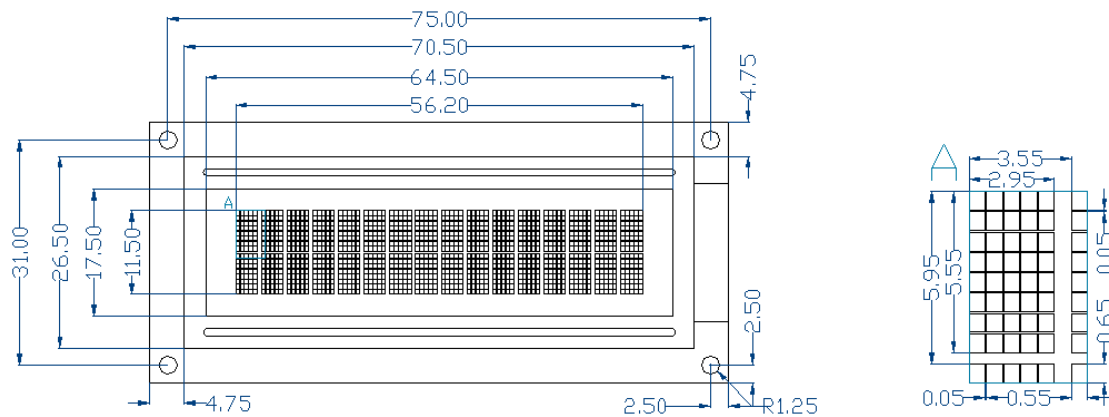
Figure 19: LK162-12 Screen Drawing
