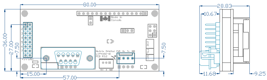
Figure 20: LK162-12 Dimensional Drawing
