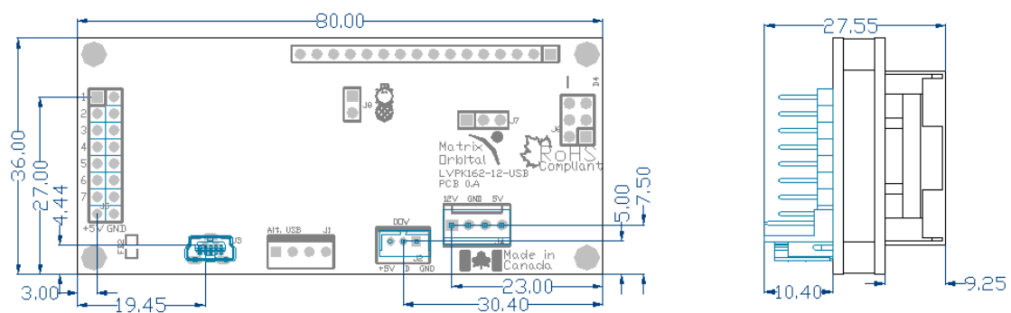
Figure 21: LK162-12-USB Dimensional Drawing
