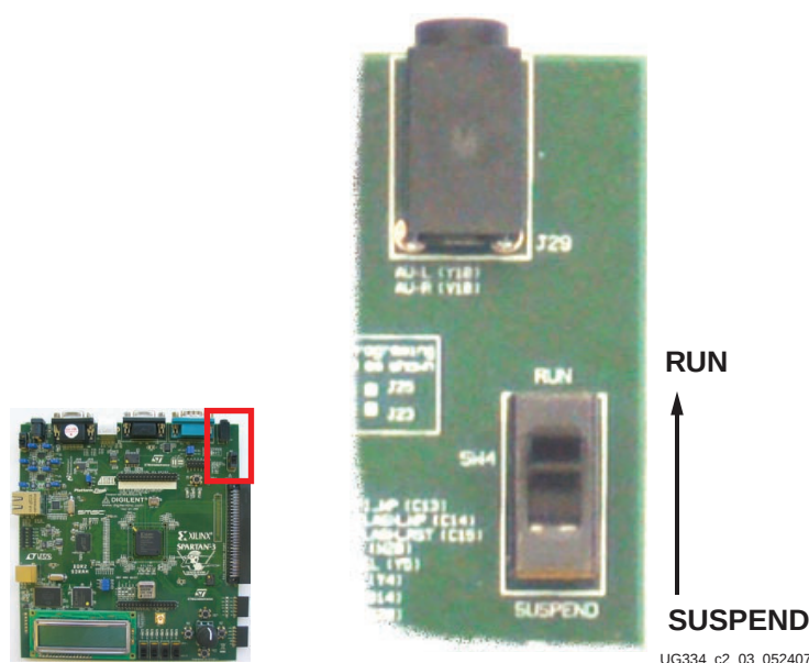
Figure 2-3: Suspend Switch
