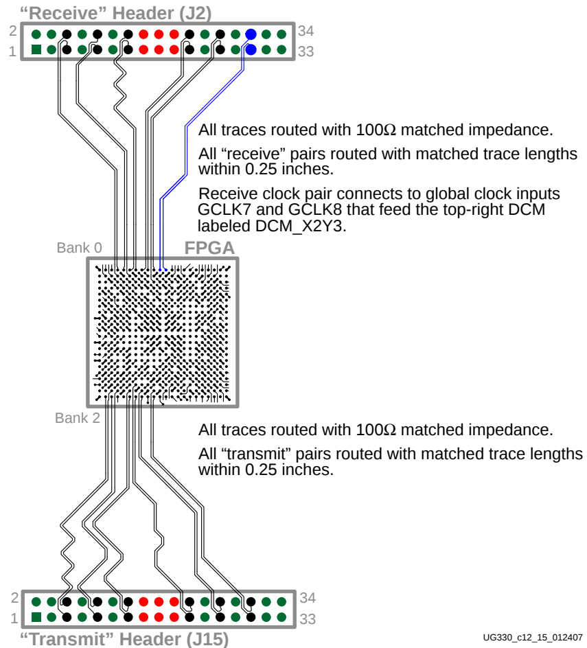
Figure 15-6: Differential I/O Layout
