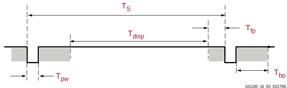
Figure 6-3: VGA Control Timing
