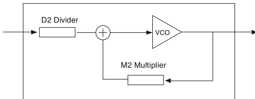
PLL2 Block Diagram
