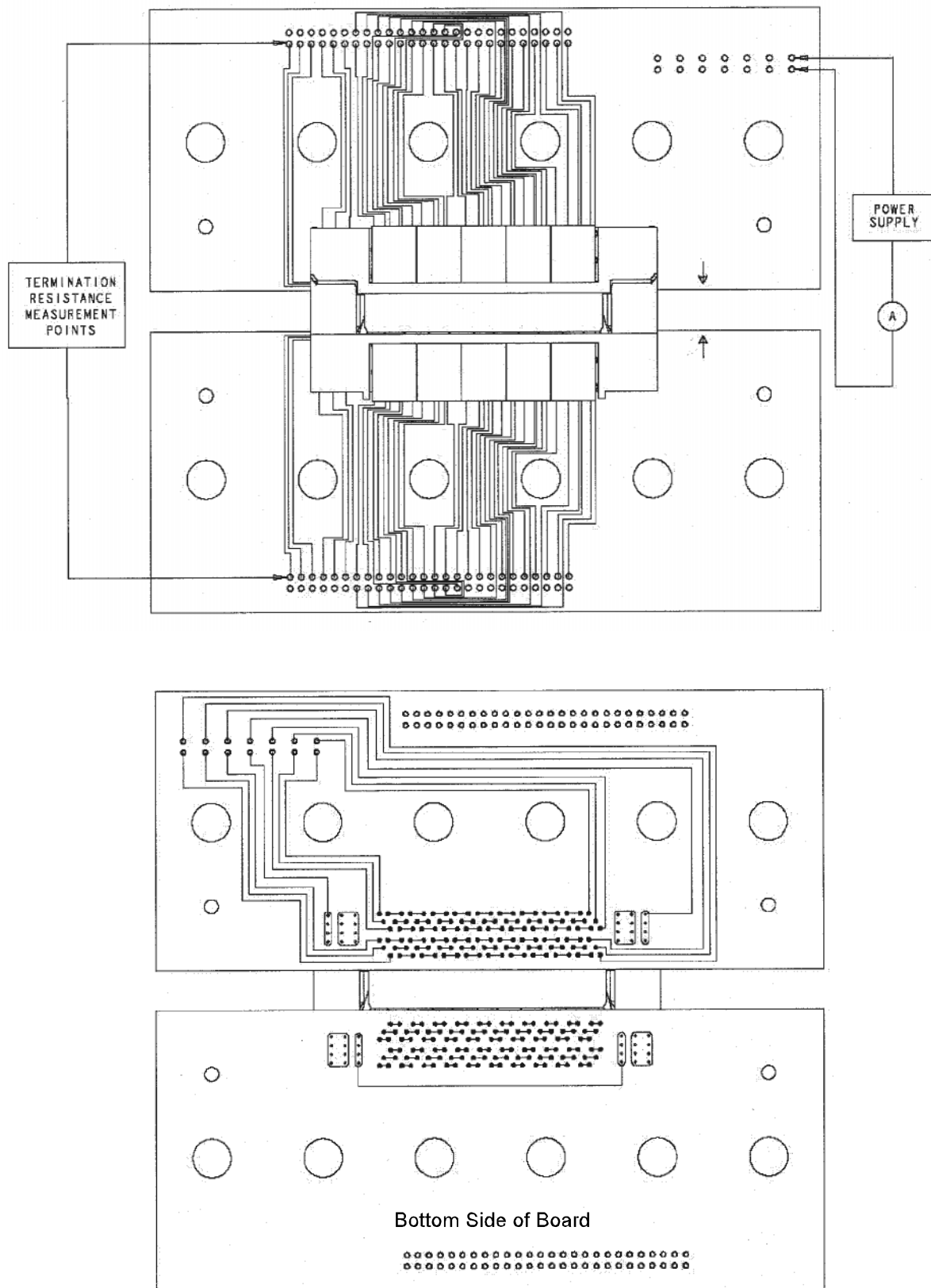
Figure 3 Low Level Contact Resistance Measurement Points
