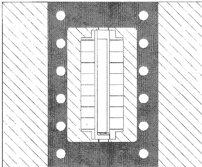
Figure 4 Vibration & Mechanical Shock Mounting Fixture
