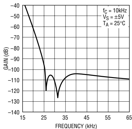
Detail of Stopband Response
