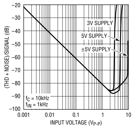
THD + Noise vs Input Voltage ( f_C = 10kHz )
