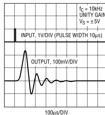
Short-Pulse Response
