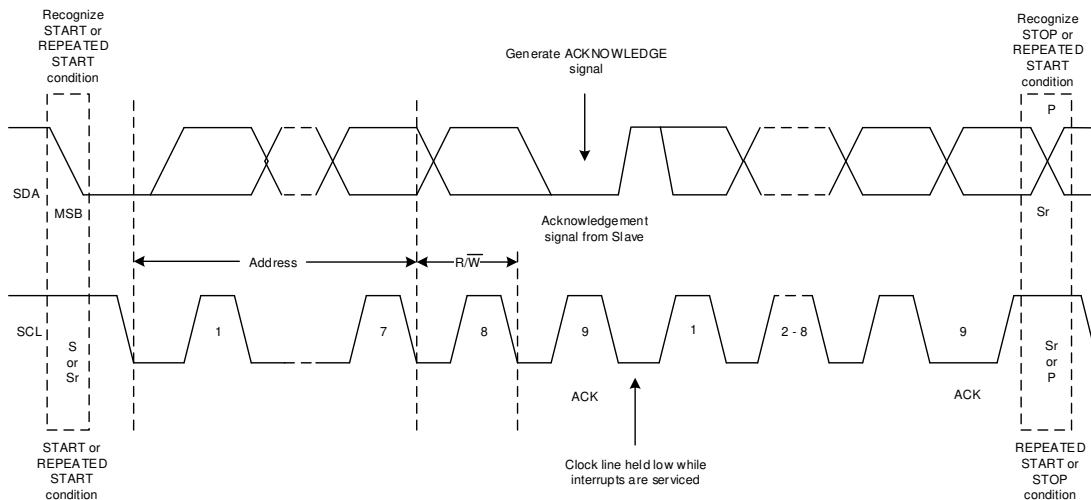
Figure 62. I 2 C Bus Protocol
