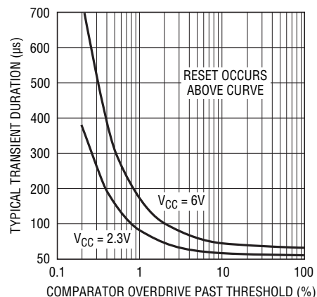
Typical Transient Duration vs Comparator Overdrive
