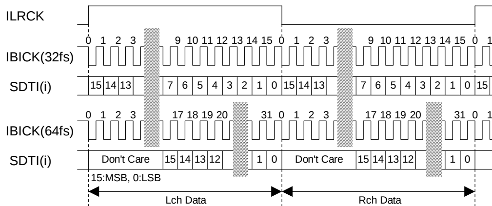
Figure 2. Mode 0 Timing
