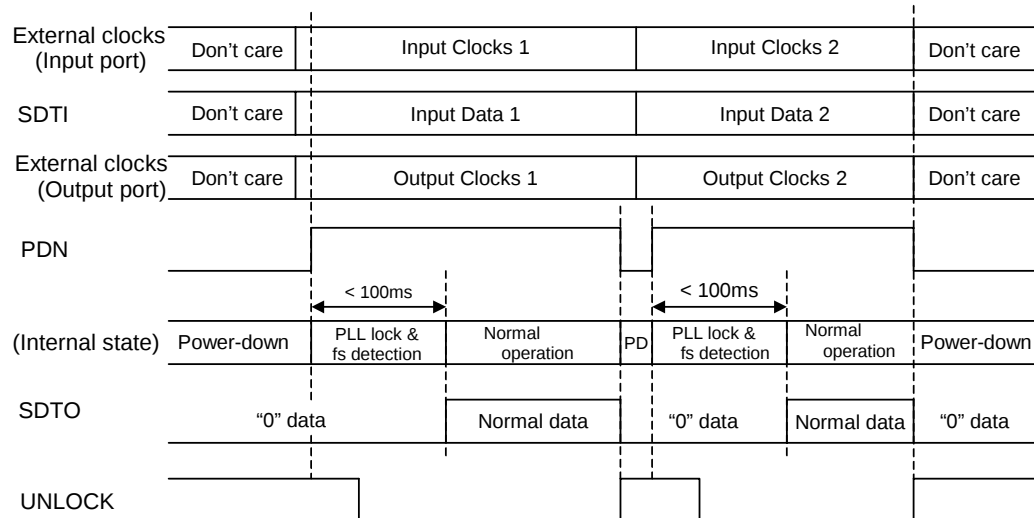
Figure 12. System Reset
