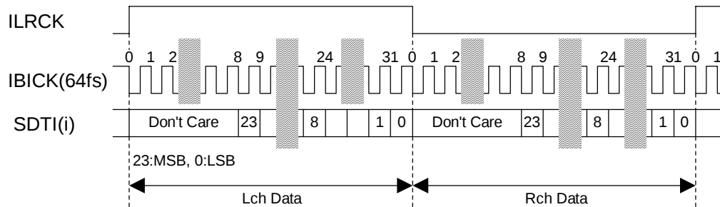
Figure 6. Mode 4 Timing
