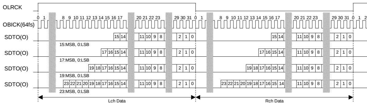
Figure 7. LSB Timing
