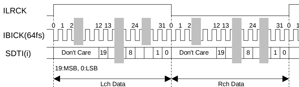
Figure 3. Mode 1 Timing
