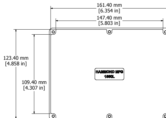
M3.5 x 0.6 (Threaded Holes) Top View Looking Inside Box
