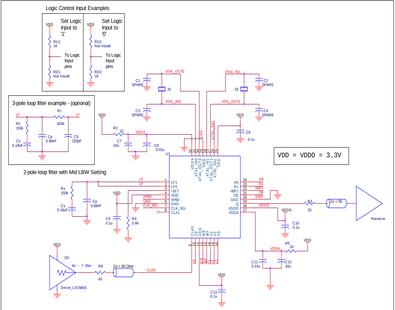
Figure 3. 810001-22 Schematic Example
