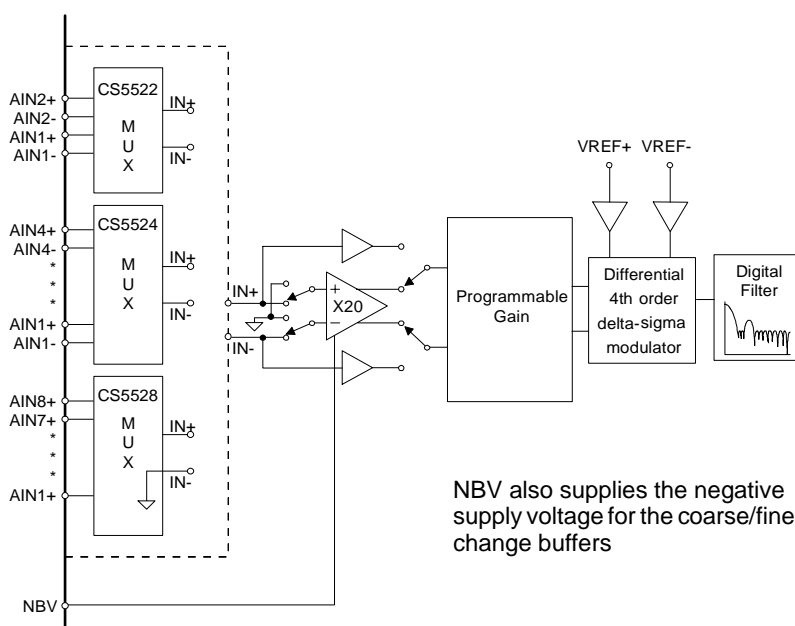
Figure 4. Multiplexer Configurations
