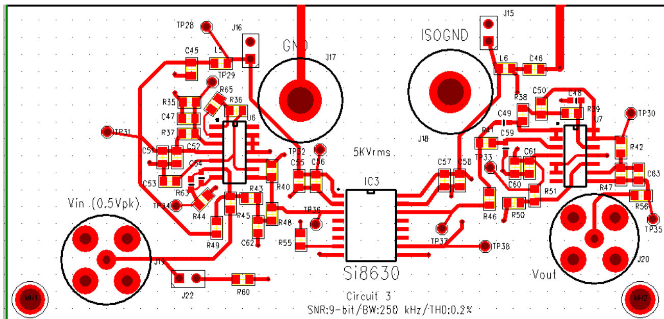
Figure 5. Circuit 3 Interface
