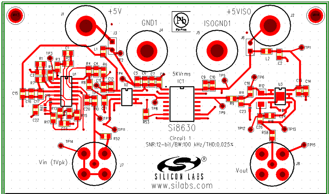
Figure 3. Circuit 1 Interface
