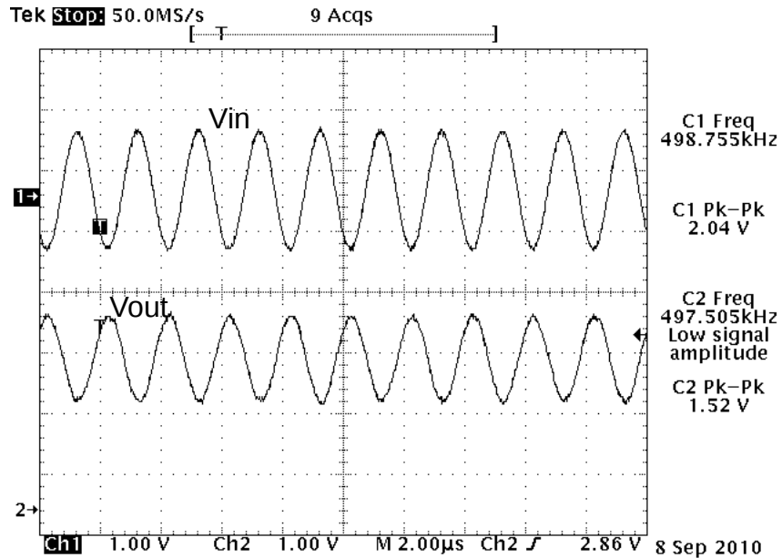
Figure 13. Circuit 2 Waveform ( V_{in} = 2 \text{ Vpp} , 500 kHz (-3 dB BW))
