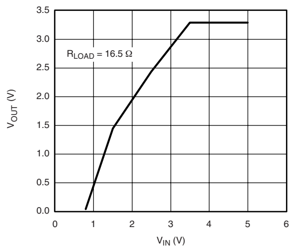
Dropout Characteristic
