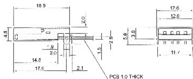
DIP
