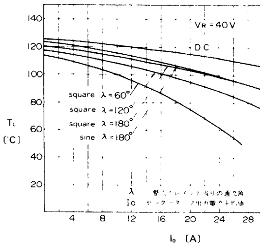
Output Current-Case Temperature
