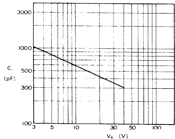
Junction Capacitance Characteristics
