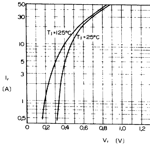
Forward Characteristics
