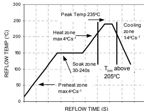
Figure 18. Reflow Profile for Tin/Lead (Sn/Pb) process.
