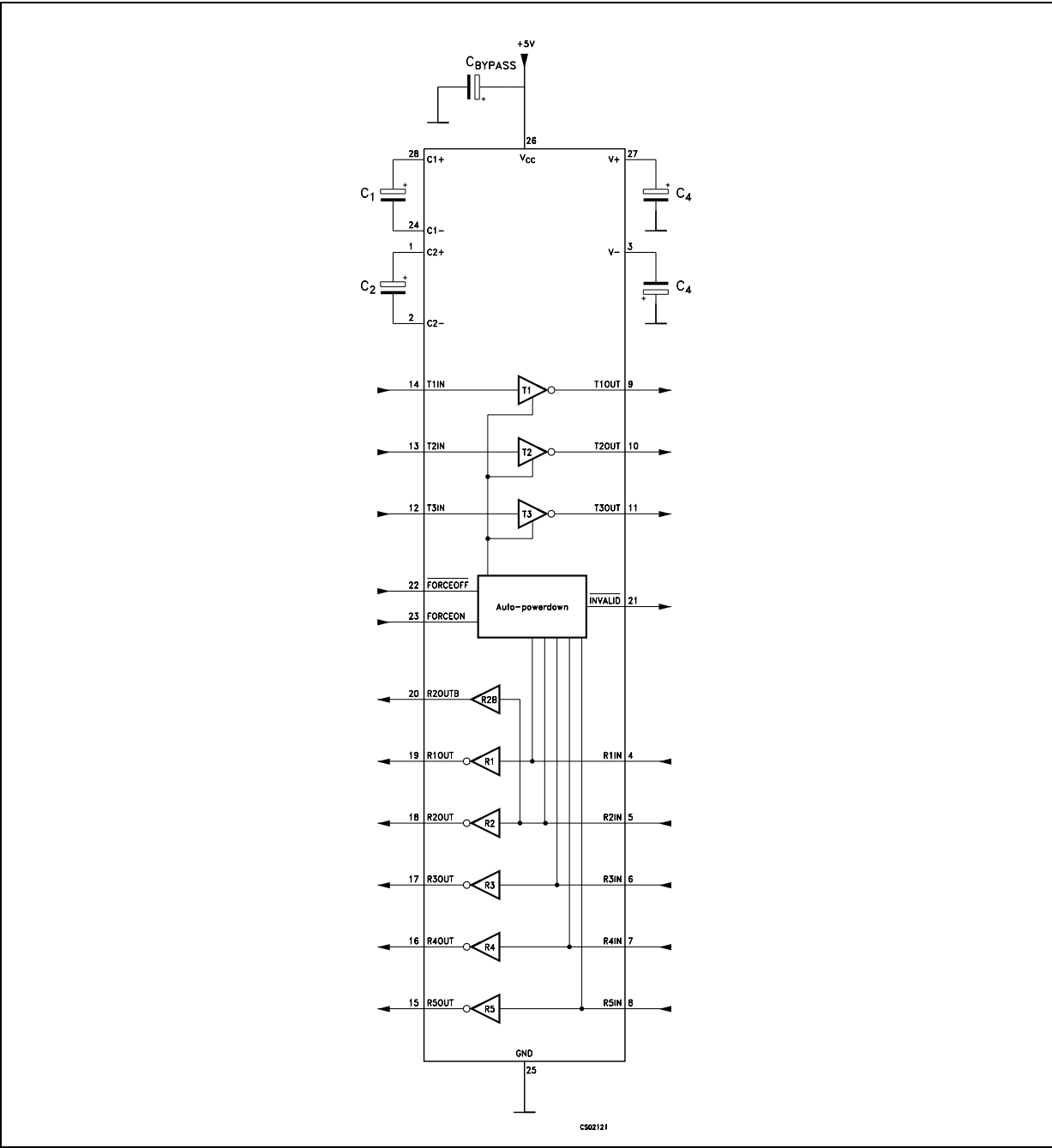
Figure 2. Application circuits
