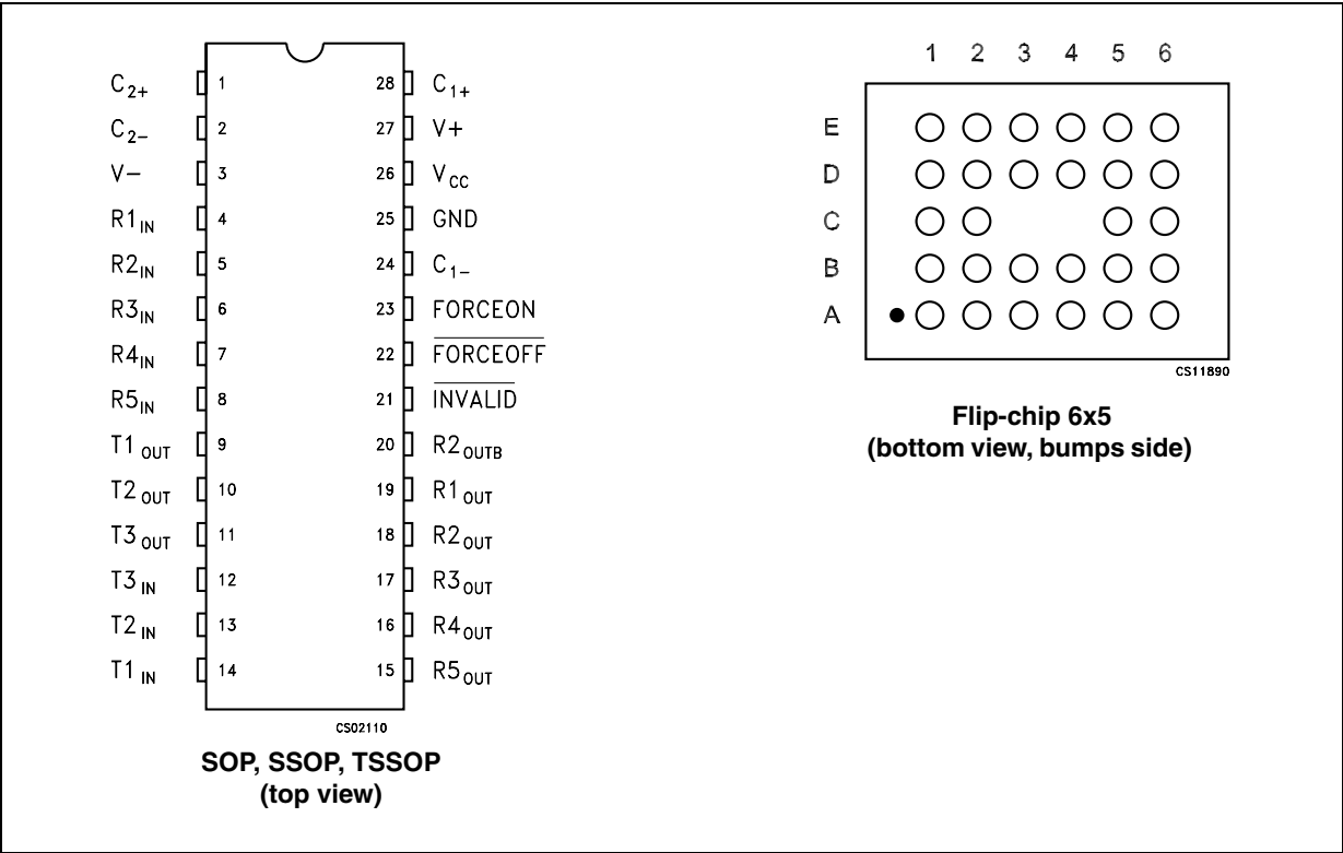
Figure 1. Pin configuration
