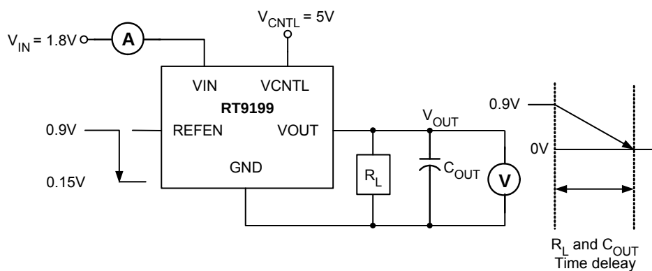
Figure 2. Current in Shutdown Mode, I_{STBY}
