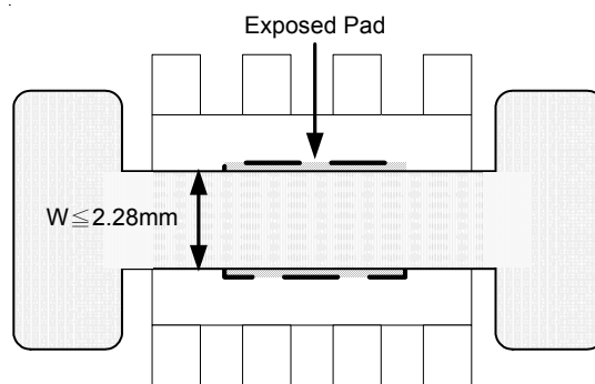
Figure 11. Dog-Bone Layout
