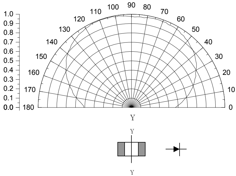
Radiation Diagram
