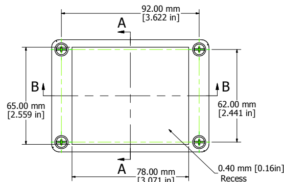
ASSEMBLY - TOP
